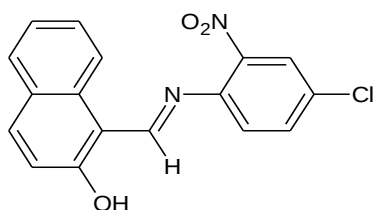
Fig. 2 Secondary ligand 1-[(E)-[(4-chloro-2-nitrophenyl)imino]methyl]naphthalen-2-ol
