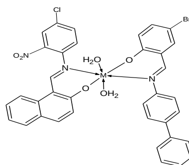
M = Co(II), Ni(II), Cu(II) and Zn(II)
