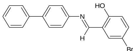
Fig. 1 Primary ligand 2-[(E)-(biphenyl-4-ylimino)methyl]-4-bromophenol
