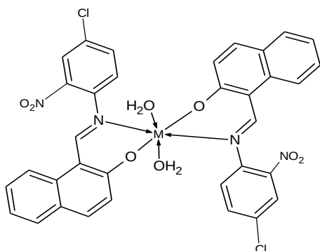
Fig. 3 The metal-ligand binary binding proposed structure
